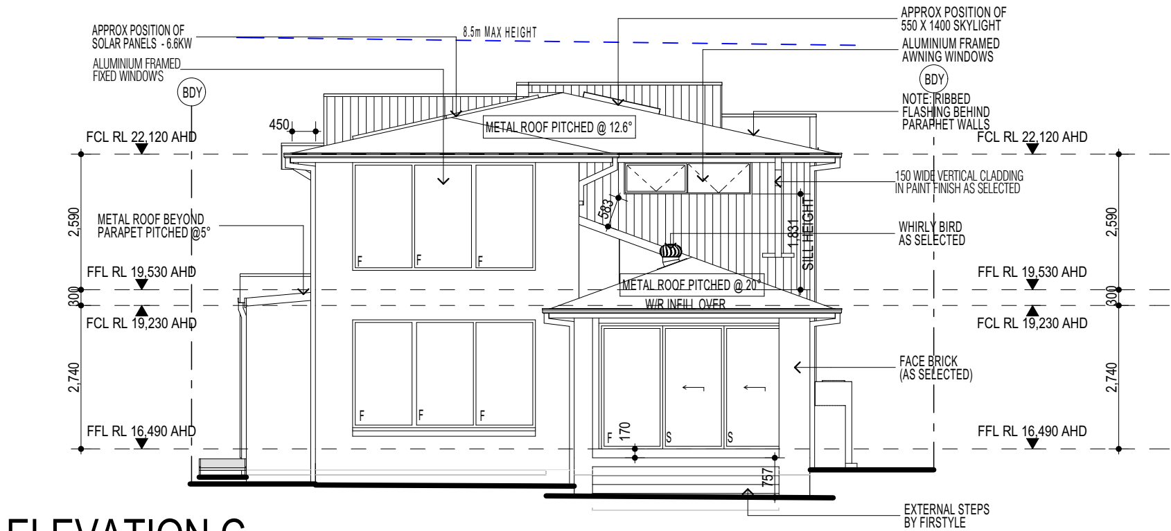
ELEVATION C
