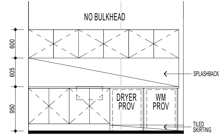
L'DRY ELEVATION SCALE 1:50
