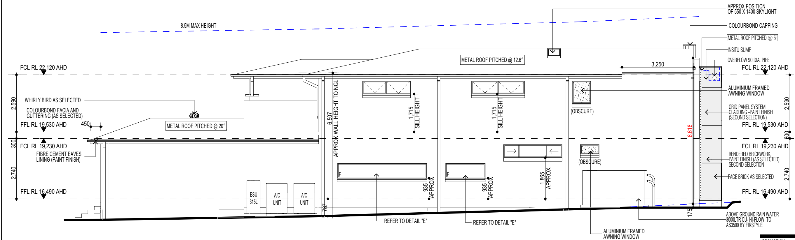
ELEVATION D
