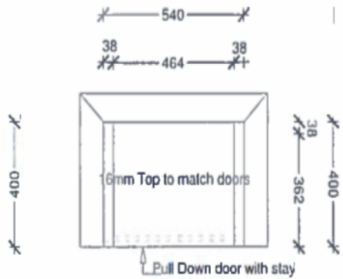
Main Bathroom Chute Cupboard
