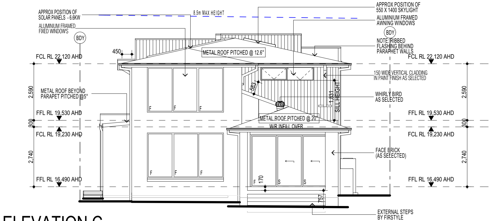
ELEVATION C
