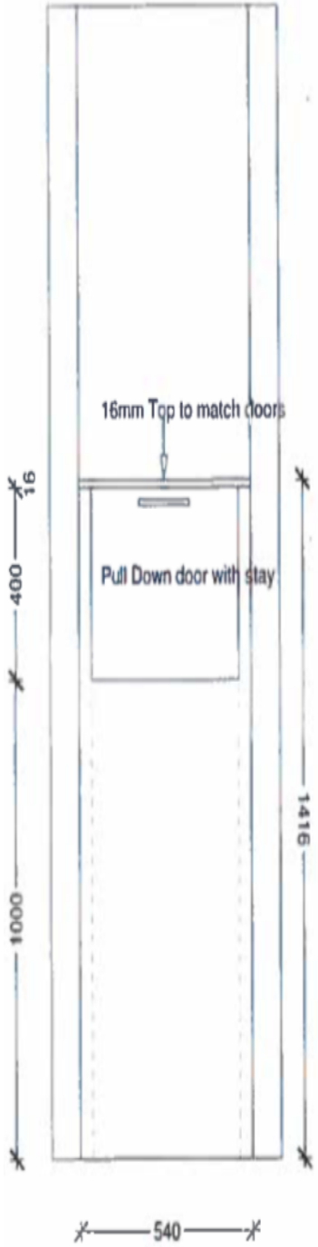
DETAIL R LAUNDRY CHUTE - NTS
